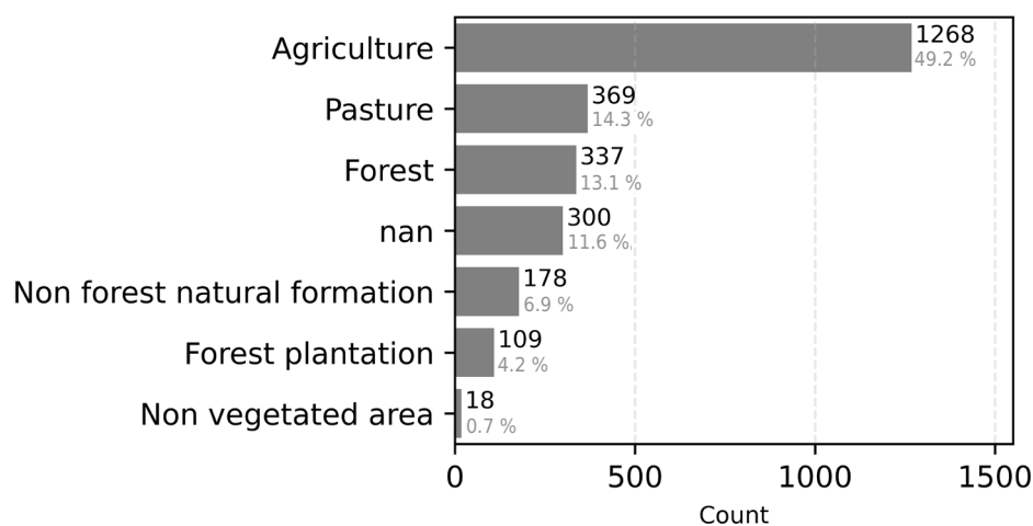
Figure 4. Distribution of the Ksat-SSIR-DB in the land use classes, according to MapBiomass (MapBiomass Project, 2022). nan indicates that there is no data representation.
