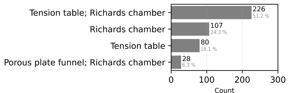
Figure 5. Methods for determining water retention of soil samples from the Ksat-SSIR-DB.
