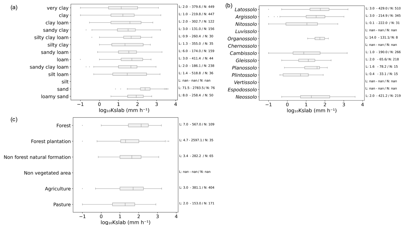
Figure 6. Box-plots of Kslab data by textural classes (a), soil classes in the first categorical level of SiBCS (b); and land use and cover classes according to MapBiomass (c). Values indicated on the right side of the graphs represent the 10th and 90th percentiles of Kslab values (mm h -1 ) in each grouping (L). Next to these values is indicated the number of soil samples included in each group (N). Groups with a number of samples less than or equal to 5 did not have data presented. nan indicates that there is no data representation.
